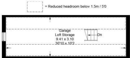
Garage First Floor
