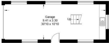
Garage Ground Floor
